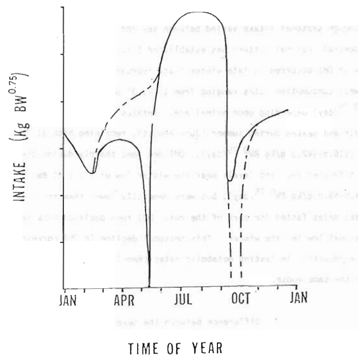
Fig. 1. Schematic drawing of seasonal intake in moose; females are represented by solid line, males by dashed line when they differ from females.
