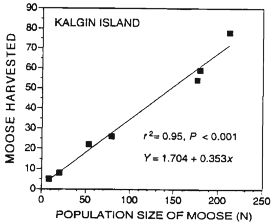
Fig. 3. Relation between number of moose harvested and their estimated population size on Kalgin Island, Cook Inlet, USA, 1981-1987. Despite the large amount of variance explained in harvest by population size, harvest alone should not be used as an index to population size.
