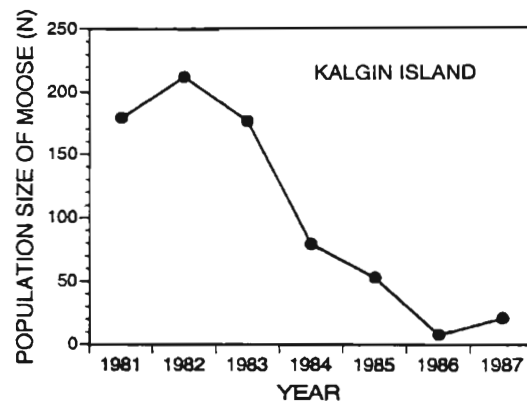
Fig. 1. Estimated population size ( N ) of Alaskan moose on Kalgin Island, Cook Inlet, Alaska, USA, from 1981 to 1987. Population sizes were estimated annually from reconstructions based on age structure of harvested moose.
