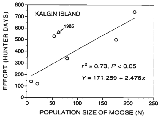
Fig. 2. Relation between hunter effort and estimated population size of moose on Kalgin Island, Cook Inlet, Alaska, USA, 1981-1987. Note the high effort relative to population size in 1985.
