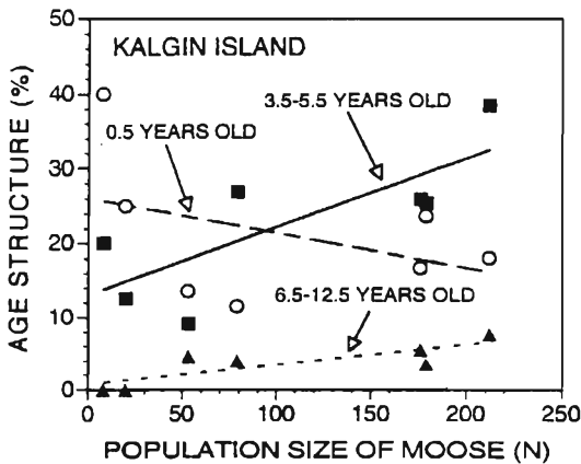
Fig. 6. Changes in age structure of moose with increasing population size, Kalgin Island, Cook Inlet, Alaska, USA, 1981-1987. Open circles = 0.5 years old, closed squares = 3.5 – 5.5 years old, and closed triangles = 6.5 – 12.5 years old. Note the increase in older age classes and decline of young moose with increasing population size.
