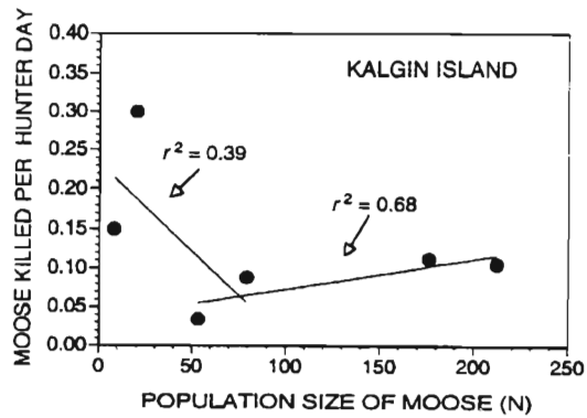
Fig. 4. Catch per unit effort (moose killed per hunter day) in relation to estimated population size on Kalgin Island, Cook Inlet, Alaska, USA, 1981-1987. Piece-wise regression indicated a change in direction for this relationship at a population size of about 75 moose.
