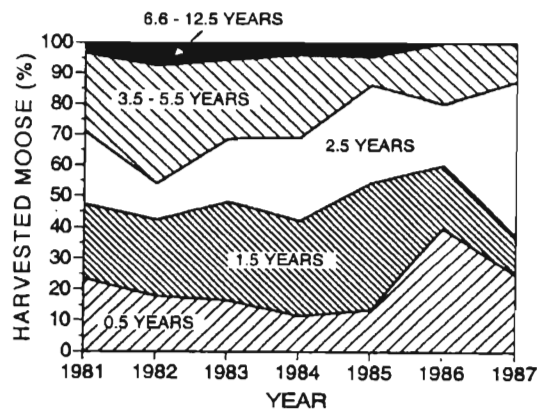
Fig. 5. Age structure of moose harvested on Kalgin Island, Cook Inlet, Alaska, USA, 1981-1987. Note the decline in older age classes through time.
